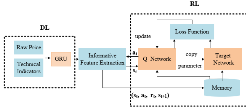
Fig. 2: The framework of GDQN.
