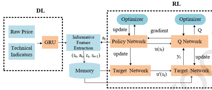
Fig. 4: The framework of GDPG.
